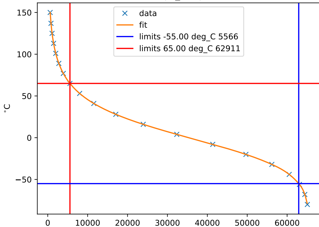
hvps_temp
